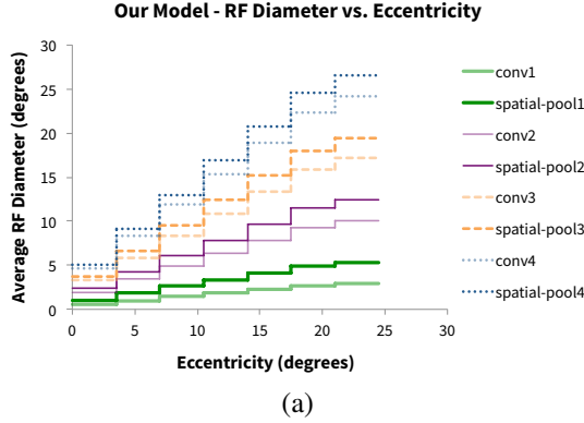
Figure 2: (a) Average receptive field (RF) diameter vs. eccentricity in our computational model. (b) Measured RFs of macaque monkey neurons—figure is from (Freeman and Simoncelli 2011).
