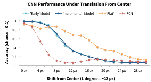
Figure 4: CNN performance under translation from center.
