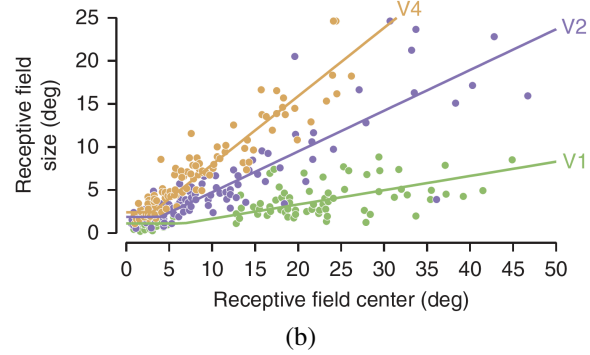
Figure 2: (a) Average receptive field (RF) diameter vs. eccentricity in our computational model. (b) Measured RFs of macaque monkey neurons—figure is from (Freeman and Simoncelli 2011).
